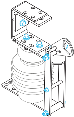
ISOMETRIC VIEWS
