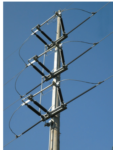
The Superwhip™ on a 115 kV phase-over-phase V2-CA switch
